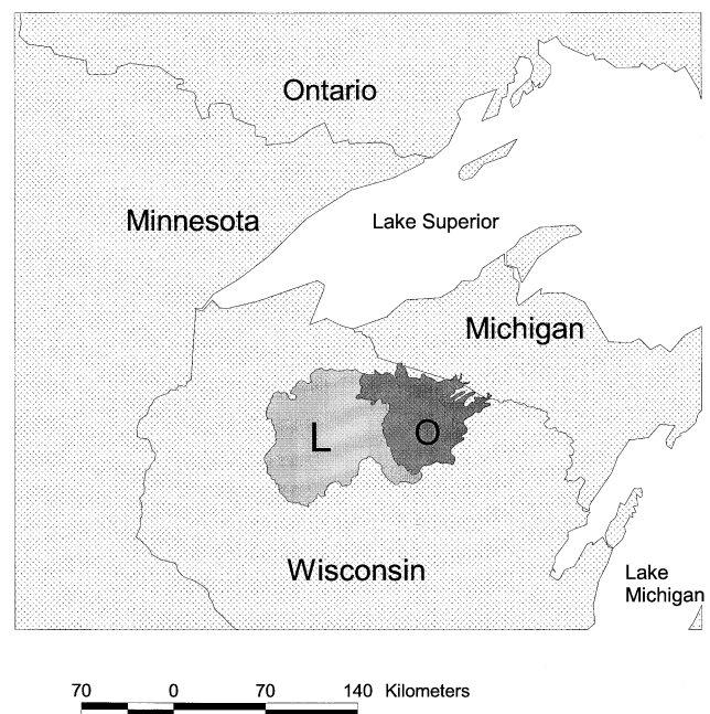
Fig. 1. Outwash plain (O) and loess plain (L) ecoregions in North Wisconsin, USA.
