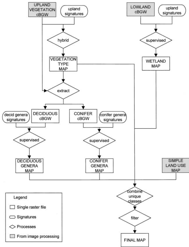
Fig. 3. Hierarchical classification steps using cBGW for the outwash plain as an example.
